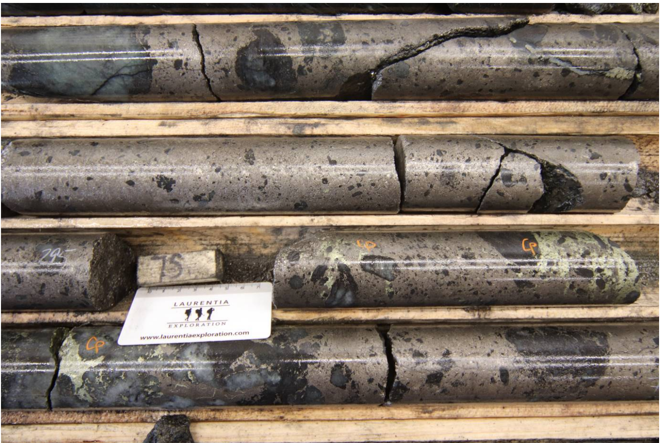
Figure 4: Zoomed in core photo of GRL-22-61 showing the massive sulphides.
